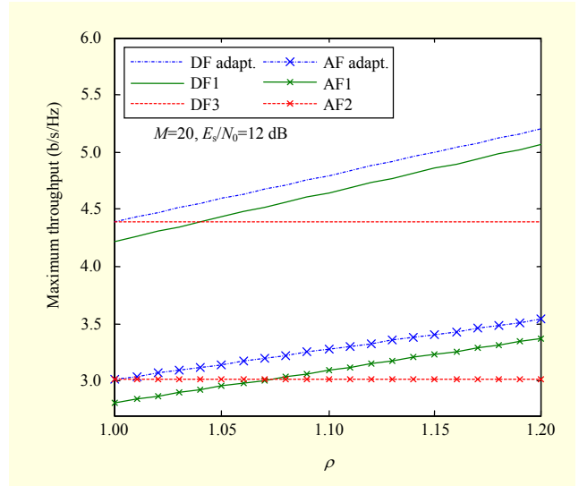
Fig. 8. Maximum throughput when DF-HARQ (AF-HARQ) is adaptively selected according to network topology.
