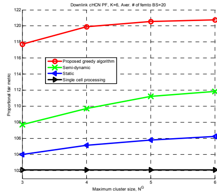
Fig. 3. Proportional fair metric for N^G=3,4,5 when N^F=20, K=6 .
